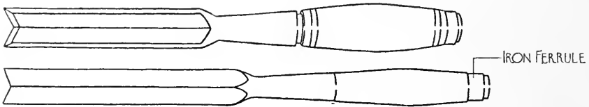
FIG. 49. CORNER CHISELS.
